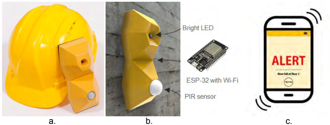
Figure 3. NoFall – Construction Site Fall Prevention System. Figure 3a. Helmet and ISCU. Figure 3b. ISCU – In Site Computation Unit. Figure 3c. Mobile app.
